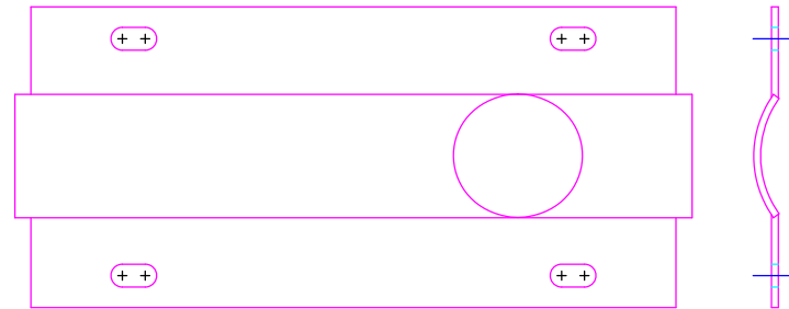
TI-255-B, COVER WITH LUBRICATION PORT.
