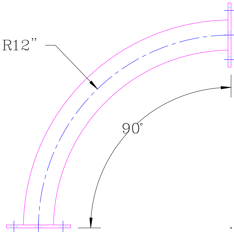
TOP VIEW
