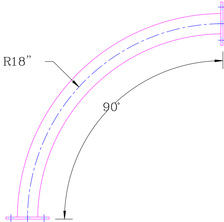
TOP VIEW
