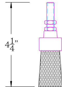
ITEM 3 LUBRICATOR BRUSH (NYLON BRISTLES)
