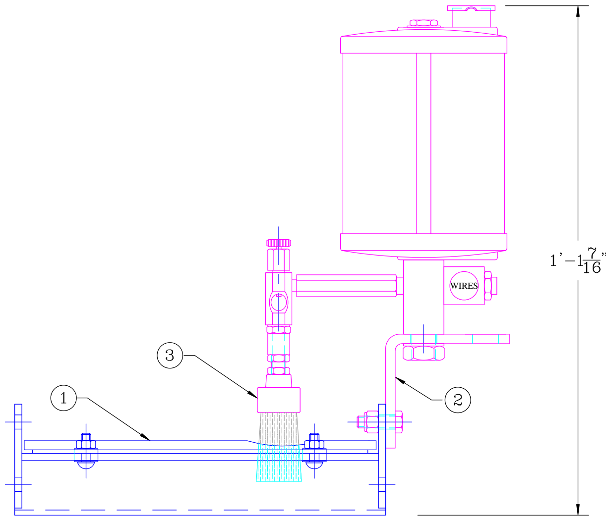
ITEM 3 LUBRICATOR BRUSH (STAINLESS STEEL BRISTLES)
