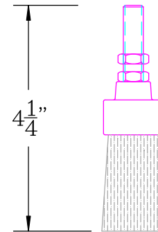
ITEM 3 LUBRICATOR BRUSH (STAINLESS STEEL BRISTLES)
